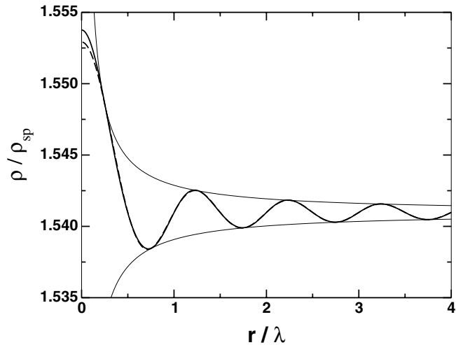
Fig. 8. Density profile for a weak oscillation \Delta x_0 = 0.7 nm (same simulation as in Fig. 6). We are still in the linear regime. The thin solid lines indicate a fit of the amplitude by 1/r and the dashed line a fit by \sin(kr)/(kr) . The latter is almost identical to the numerical result, except near the focal point where nonlinear effects become visible. The simulation was done with 100 mesh points per wavelength, starting with a static density \rho_{st} = \rho_0 and thus a vanishing static pressure.
