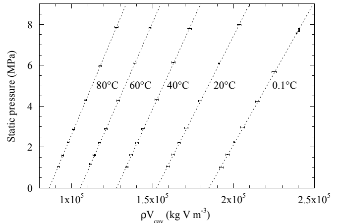
FIG. 13: Static pressure as a function of the product \rho V_{\text{cav}} for 5 of the 15 temperatures investigated in run 0. The dotted lines are linear fits to the data; each set is labelled (on the right) with the temperature. Experimental error bars are shown on each data point; most of the vertical errors are too small to be seen at this scale.
