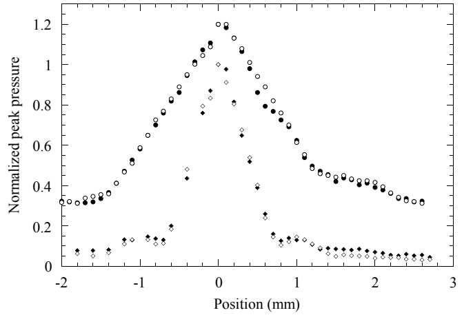
FIG. 11: Map of the acoustic field. The data (normalized to 1 at the focus) were taken with a 40\ \mu\text{m} needle hydrophone in an open container at room temperature ( \simeq 25^\circ\text{C} ), using 1-cycle bursts. Filled (resp. empty) symbols correspond to the maximum (resp. minimum) pressure in a burst. Diamonds (bottom) show a scan in the equatorial plane of the transducer, whereas circles (shifted by 0.2 for clarity) show a scan along its axis.
