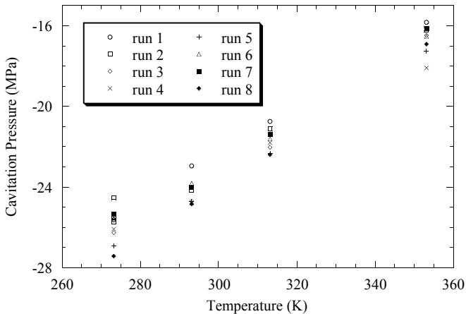
FIG. 18: Cavitation pressure as a function of temperature, obtained with the static pressure method (see Sec. IV D), for runs 1 to 8. The error bars are omitted for clarity; they are similar to those in Fig. 15.
