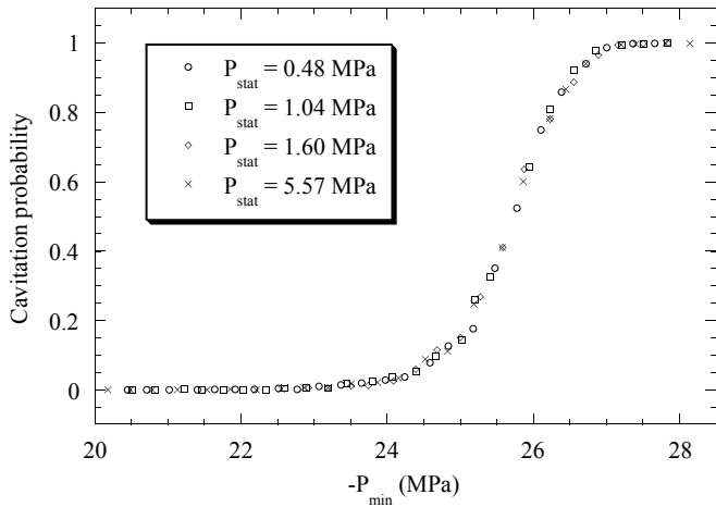
FIG. 16: Cavitation probability as a function of the minimum pressure reached in the wave for 4 different static pressures. Each point is an average over 1000 bursts. The data were taken during run 0 at T = 4^\circ\text{C} .
