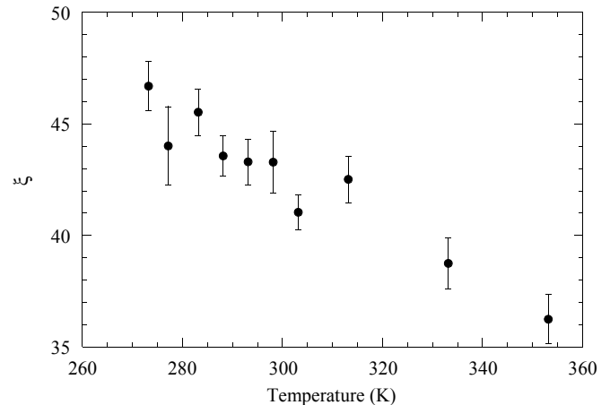
FIG. 17: Steepness of the S-curves as a function of temperature. Each data was measured in run 0, using 25 points with statistics over 1000 bursts, at P_{\text{stat}} = 1.6 \text{ MPa} .
