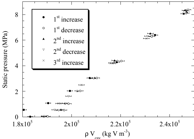
FIG. 14: Static pressure as a function of the product \rho V_{\text{cav}} during the first pressure cycles of run 3 at 0.1 °C.
