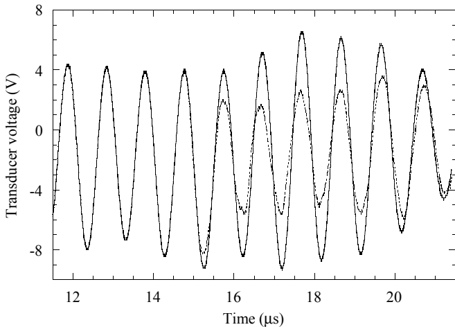
FIG. 7: Relaxation voltage of the transducer. The two traces were recorded for two successive 4-cycles bursts with the same experimental conditions ( T = 20^\circ\text{C} , P_{\text{stat}} = 1.7\text{ MPa} , V_{\text{cav}} = 163.3\text{ V} ). The solid line corresponds to the reproducible relaxation signal of the transducer coming back to rest, without cavitation. The dashed line is an example of the random echo signal reflected on the nucleated bubble and reaching the transducer voltage with a delay t_f after nucleation.
