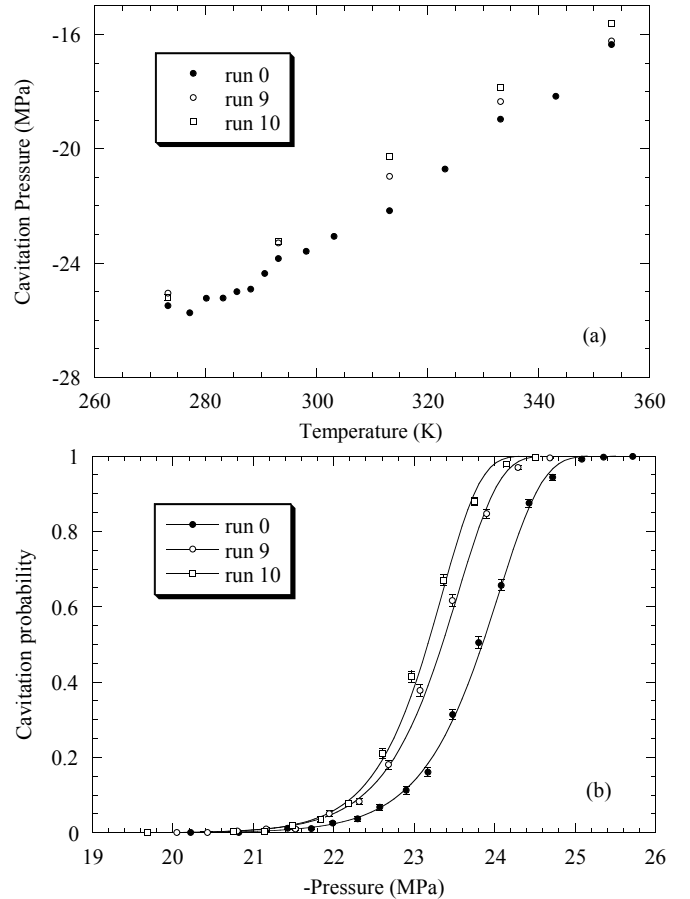
FIG. 21: Comparison between different water samples. The initial run (run 0, filled circles, as in Fig. 15) is shown for comparison. In run 9 (empty circles), we used ultrapure water from a different source (G Chromasolv for gradient elution, purchased from Sigma), and degassed with the method described in Sec. III F. In run 10 (empty squares), we used mineral water (Speyside Glenlivet, dry residue at 180^\circ\text{C} : 58 \text{ mg L}^{-1} ) [61], distilled in a Pyrex glassware and degassed with the same method. (a) Cavitation pressure as a function of temperature; the error bars on P_{cav} are omitted for clarity: they all have a similar amplitude (see Fig. 15). (b) Cavitation probability as a function of the minimum pressure reached in the wave. The S-curves were obtained at T = 20^\circ\text{C} and P_{\text{stat}} = 1.6 \text{ MPa} . The excitation voltages were converted into pressure using Eq. 11 and the value of P_{cav} shown in (a). The solid curves are fits with Eq. 12; they all give similar values of the steepness \xi : 43.3 \pm 1 for run 0 ( \chi^2 = 2.2 ), 44.6 \pm 1.5 for run 9 ( \chi^2 = 3.9 ), and 48.1 \pm 1.9 for run 10 ( \chi^2 = 4.6 ).
