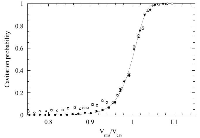
FIG. 23: Cavitation probability as a function of the excitation voltage normalized to the cavitation voltage. Full (resp. empty) circles stand for ultrapure (resp. tap) water. The data were recorded at room temperature in an open Pyrex glass container. Each point corresponds to 1000 repeated bursts. The solid line is a fit of the data for ultrapure water with Eq. 9. The center of these S-curves are similar, but the foot for tap water is much broader than for ultrapure water. This indicates the presence in tap water of a broad distribution of dilute impurities triggering cavitation at pressures less negative than the cavitation pressure of ultrapure water.
