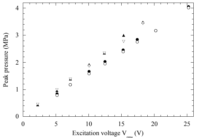
FIG. 12: Peak pressures measured by the hydrophones as a function of the transducer excitation voltage. The data were taken in an open container at room temperature ( \simeq 25^\circ\text{C} ), with 4-cycles bursts, the cavitation threshold voltage being V_{\text{cav}} = 130\ \text{V} . Filled (resp. empty) symbols correspond to the maximum (resp. minimum) pressure in a burst. Circles (resp. triangles) were obtained with a 40\ \mu\text{m} (resp. 200\ \mu\text{m} ) needle. The manufacturer gives a calibration uncertainty on the gain of 14%, which means that the results from the two needles are consistent with each other.
