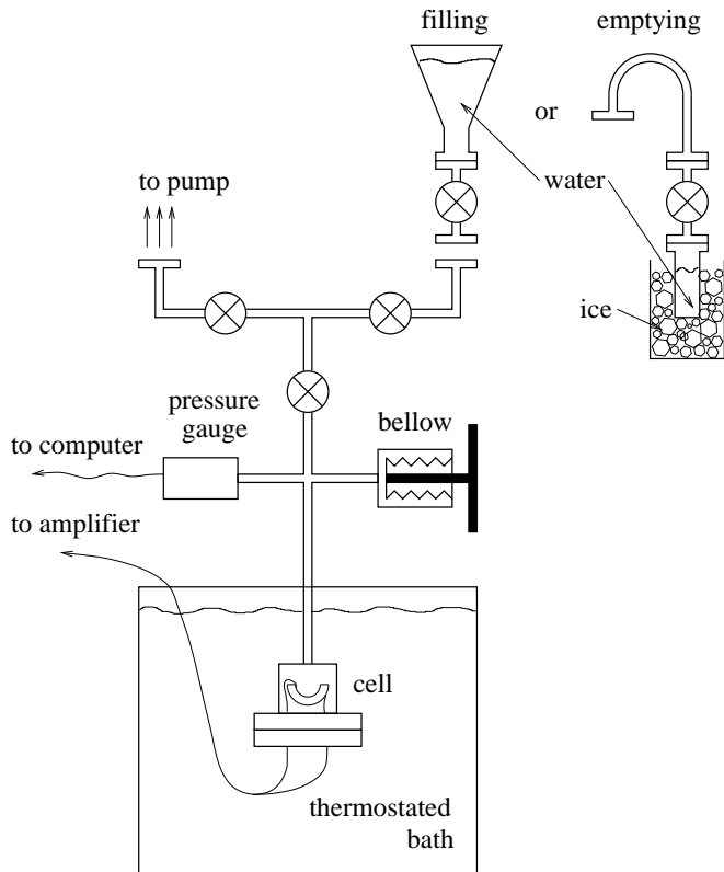
FIG. 5: Sketch of the experimental setup. The high pressure part contains the cell with the transducer, the pressure gauge and the bellow for pressure control; it can be isolated from the rest by a valve. The use of two other valves allows evacuation (with an oil pump through a nitrogen trap or a dry scroll pump), filling (the flask with degassed water being connected), and emptying (the collecting vessel being connected and cooled with ice). The cell is immersed in a thermostated bath (operated between -10 and 80^\circ\text{C} ). All the seals are made of SS or bulk Teflon, except the one at the bottom of the cell, which is made with an indium wire.
