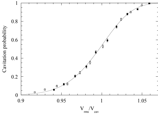
FIG. 20: Cavitation probability as a function of the excitation voltage normalized by the cavitation voltage. Each filled (resp. empty) circle shows the probability measured with a 1 MHz (resp. 1.3 MHz) transducer, by counting the cavitation events over 1000 bursts, at room temperature in an open Pyrex container. A fit with Eq. B8 (solid line), using P_2/P_{cav} = 0.8 and \alpha = 11/2 , give n_0\lambda^3 [P_{cav}/(P_2 - P_1)]^{13/2} = (3.62 \pm 0.10) 10^7 for both frequencies.
