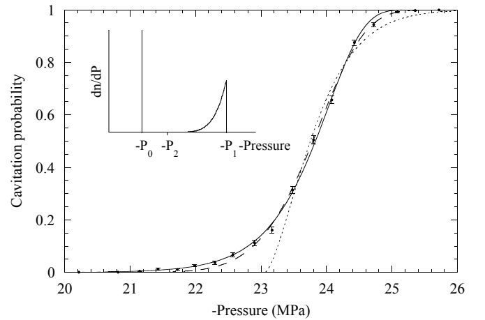
FIG. 25: Cavitation probability as a function of the minimum pressure reached in the wave. The data points are the same as in Fig. 9. The excitation voltage has been converted into pressure using Eq. 11 and P_{\text{cav}} = -23.845 MPa. Only pressures between -20 and -26 MPa are shown. The solid line is a fit with Eq. 12. The best fit gives -P_{\text{cav}} = 23.847 \pm 0.019 MPa and \xi = 43.3 \pm 1 with \chi^2 = 2.2 . The inset shows the two distributions of type II impurities tested (see Appendix B). Eq. B6 (corresponding to the monodisperse distribution) does not allow a good fit; the dotted line is drawn with P_0 = -23 MPa and n_0\lambda^3 = 600 to pass through the high probability data. The dashed line is a fit with Eq. B8; P_2 was set to -20 MPa, and the best fit was obtained for \alpha = 5 : it gives n_0\lambda^3/(P_2 - P_1)^6 = (0.31 \pm 0.01) MPa ^{-6} and \chi^2 = 3.7 .
