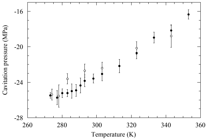
FIG. 15: Cavitation pressure as a function of temperature. P_{\text{cav}} was obtained with the static pressure method (see Sec. IV D). Run 0 (filled circles) is compared to our preliminary results [56] (empty circles). The uncertainties on P_{\text{cav}} were calculated as described in Sec. V A.
