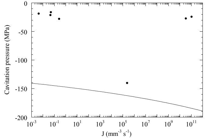
FIG. 2: Cavitation pressure as a function of the quantity J = 1/(V\tau) . Data points are listed in Table I. The solid line is the prediction of the TWA (Eq. 3).
