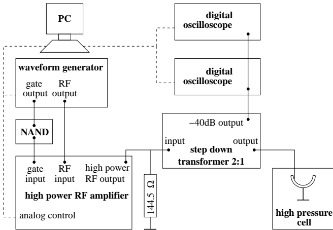
FIG. 3: Block diagram of the driving circuit of the transducer. The different units are designated in bold font. The solid lines represent the electrical connections, and the dashed lines the connections for computer control. The shunt resistor and the step-down transformer are used to improve the shape of the excitation voltage.
