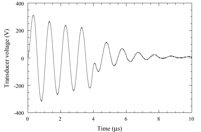
FIG. 4: Excitation voltage of the transducer, driven with a 4-cycles burst, at the cavitation threshold at T = 20^\circ\text{C} and P_{\text{stat}} = 1.7 \text{ MPa} . This corresponds to a peak power of 3.4 kW.
