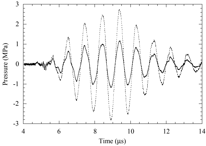
FIG. 10: Response of the 40\ \mu\text{m} needle hydrophone at the focus. The hydrophone voltage has been converted into pressure using the manufacturer's calibration data. The solid (resp. dotted) curve corresponds to an excitation voltage V_{\text{rms}} = 7.21\ \text{V} (resp. 17.42\ \text{V} ), that is 5.5% (resp. 13.4%) of the cavitation voltage. The time scale starts with the excitation voltage, and the acoustic wave reaches the focus after the time of flight over the transducer radius ( t_f = R/c , see Sec. IV A).
