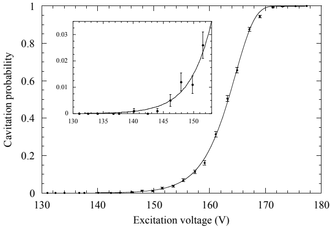
FIG. 9: Cavitation probability versus excitation voltage for 4-cycles bursts at T = 20^\circ\text{C} and P_{\text{stat}} = 1.7\text{MPa} . Each of the 25 data points was measured over 1000 repeated bursts. The standard deviation on the probability (calculated with the binomial law) is shown as error bars. The data are well fitted with Eq. 9 (solid line). The inset focuses on the low probability region, to show that zero probability is actually reached in the broad foot of the S-curve.
