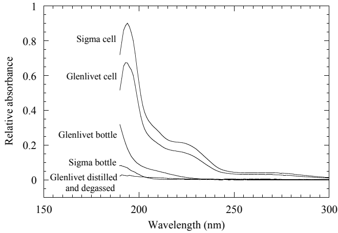
FIG. 22: UV spectra of different water samples. The labels indicate the water origin and preparation: Sigma refers to water used in run 9, and Glenlivet in run 10. Bottle is relative to the UV spectrum of water directly coming out of the commercial bottle, whereas cell refers to the water coming out of the cell at the end of the run. We also show the spectrum of Glenlivet water after distillation and degassing; these steps decrease the UV absorbance.
