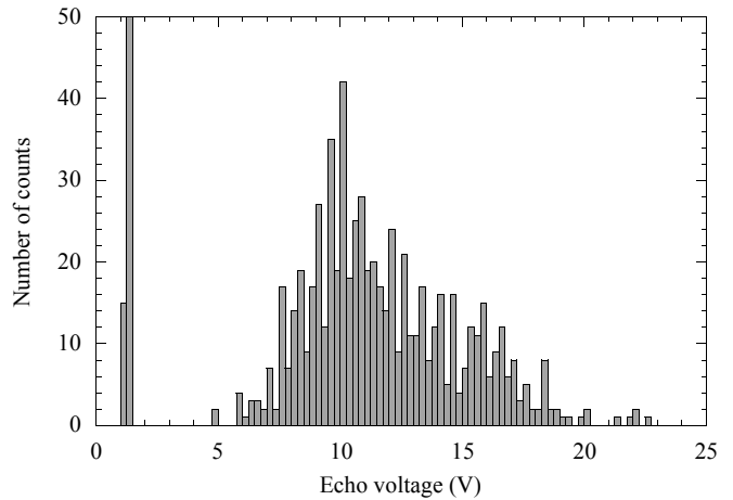
FIG. 8: Histogram of the peak-to-peak value of successive echoes. The left group of data shows the small noise on the excitation voltage without cavitation, the right one shows the various amplitudes reached by echoes with cavitation. The 1000 data points are distributed among 100 bins; the main peak (reaching 328 counts) is truncated for clarity.
