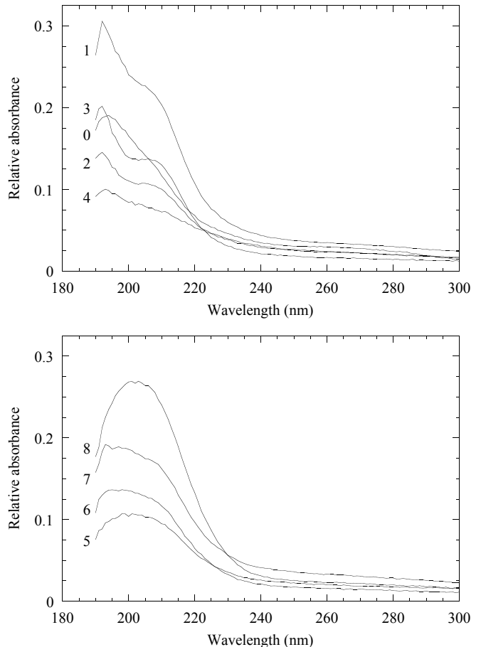
FIG. 19: UV absorption spectrum of the water collected from the experimental cell for 9 successive runs. We used an automated spectrometer (Kontron Instruments, Uvikon 941) with quartz cuvettes (10 mm thickness). The reference cuvette was filled with ultrapure water directly drawn from the water polisher and sealed with a Teflon cap. The label indicates the run number.
