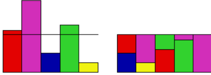
Figure 4: Walker's algorithm. (a): Distribution \{\pi_1, \dots, \pi_N\} to be sampled. Each \pi_i is represented by a slab. The mean of the \pi_i is shown. (b): Rearrangement of the slabs into a perfect rectangle, from which the sampling is straightforward.
