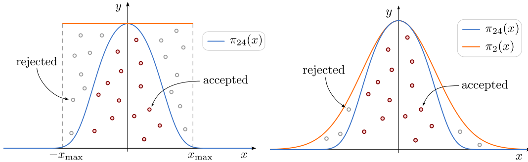
Figure 7: Naive and state-of-the-art algorithms to sample the Boltzmann distribution for the anharmonic oscillator as uniformly distributed pebbles. (a): The naive algorithm introduces a cutoff x_{\max} and discards many pebbles. (b): Sampling pebbles (x, y) below the Gaussian curve and then discarding those samples (x, y) above \pi_{24}(x) is a winning strategy (see eq. (17))
