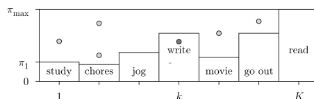
Figure 2: Saturday night problem solved by Alg. 2 ( reject-finite ).
