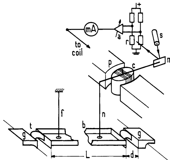
Figure 1. Schematic diagram of the transducer: (a) amplifier; (b) boom; (c) coil; (f) fixed stainless steel needle; (m) mirror; (mA) current measurement for output; (n) moving stainless steel needle; (p) poles of magnet; (r) photoresistors; (s) collimated light source; (t) Teflon tape; (g) Teflon blocks clamped on each side of the trough. This schematic diagram shows most of the features, but is not to scale. The coil bearings and the return springs of the galvanometer have been omitted for clarity. g, t, and b partition the liquid surface hermetically into two parts.
