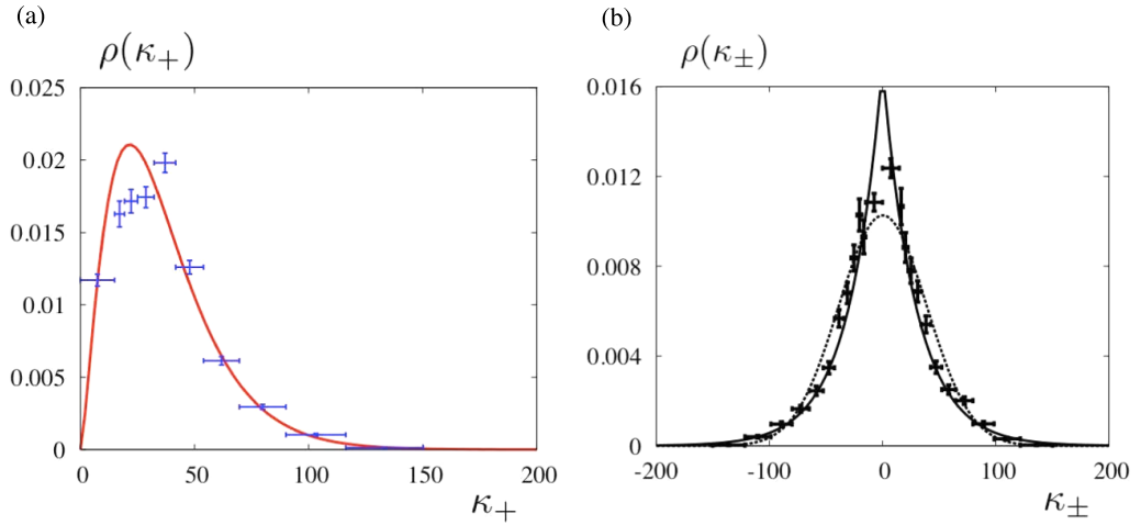
Figure 15. Simulations. Geometrical properties. (a) Probability distribution of the absolute curvature per branch \kappa_+ and Gamma distribution. The parameters for the Gamma law are \alpha = 2.5 and \chi = 14.8 . (b) Probability distribution of the curvature of branches \kappa_{\pm} with a normal distribution (dashed line) with \mu = 0 and \sigma = 39 , and an exponential distribution (continuous line) with \mu = 30 . Statistical test: \chi^2 = 93 for the exponential distribution and 160 for the normal law. Data are averaged over 4676 branches.
