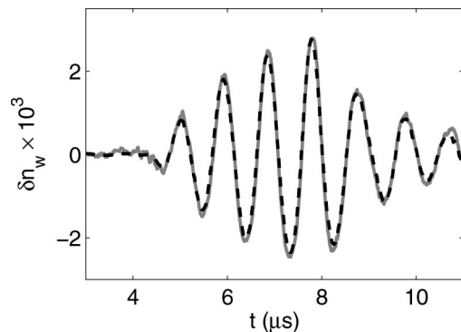
Fig. 5. Comparison of refractive index modulations obtained from the fiber-optic probe hydrophone (gray solid curve) and from inverse Abel transform of the phase map (dark dashed curve).
