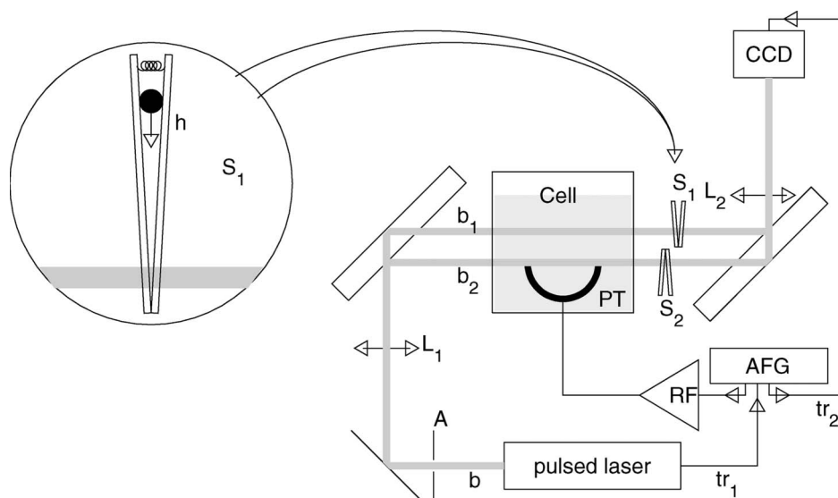
Fig. 1. Experimental setup: b, attenuated laser beam; tr1, trigger pulse sent by the laser 170 \mu\text{s} before the laser pulse; AFG, function generator; tr2, trigger pulse for the CCD camera; PT, piezo transducer driven by the amplifier RF; S_1 , scanning plates for the interferometer; S_2 , compensating plates. The inset shows how the optical path for the beam b_1 is changed by moving the separator of S_1 plates by h .
