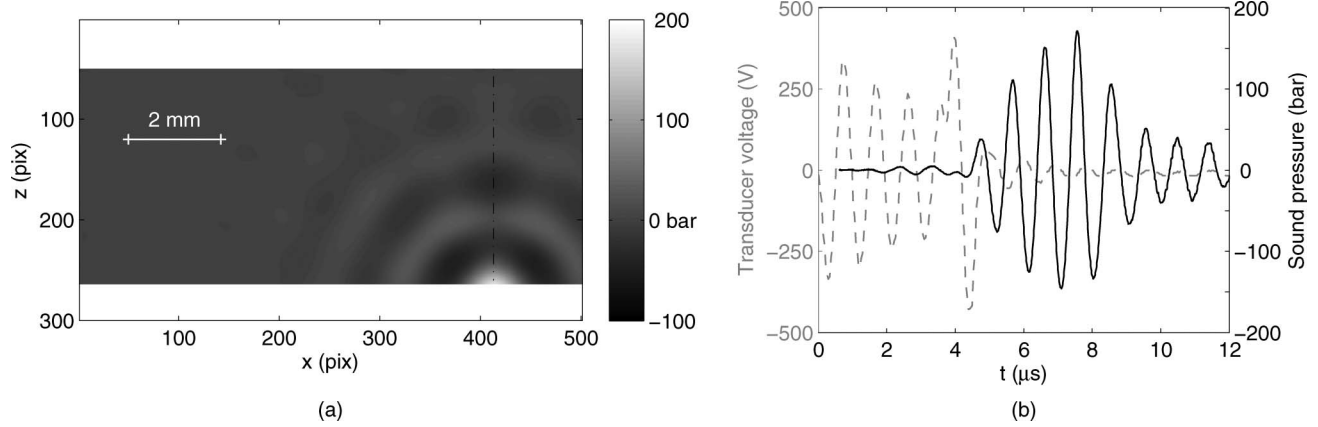
Fig. 4. (a) Pressure map computed from the phase map Fig. 3(b) by Abel inversion from pixel 1 to 414. Area from x = 414 to x = 500 are filled by symmetry. (b) Time variations of the computed pressure at the focus while the sound pulse goes through (solid curve). The transducer excitation voltage is also plotted (dashed curve), starting at t = 0 .
