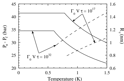
Fig. 2. Nucleation pressure of the solid as obtained from the TWA (solid lines, left scale). The radius of the critical nucleus is also shown (dashed lines, right scale). Two typical values of \Gamma_0 V \tau were used: 10^{32} (corresponding to the large cell experiment) and 10^{17} (corresponding to the ultrasonic experiment).
