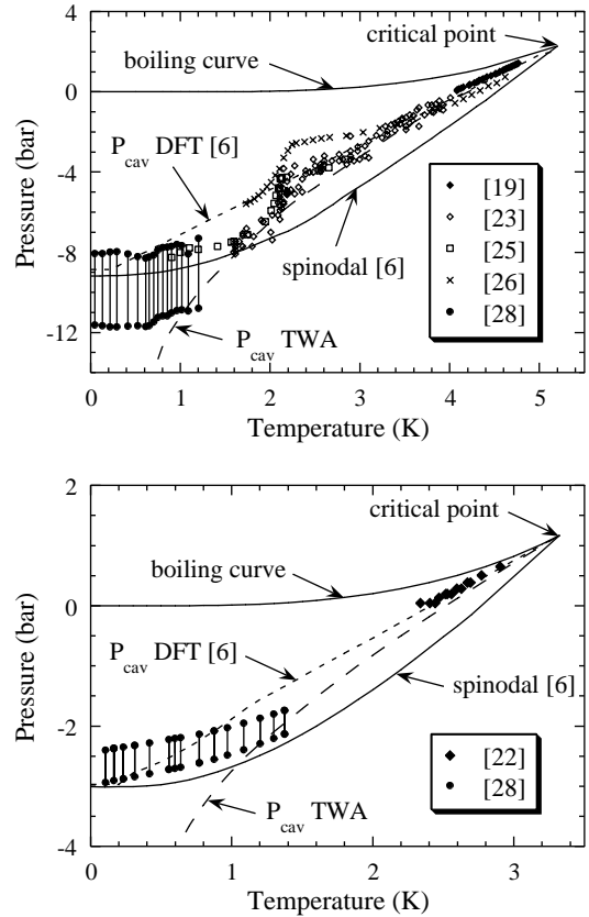
Fig. 1. Compilation of theoretical (dashed lines) and experimental (data points) values of P_{cav} in ^4\text{He} (top) and ^3\text{He} (bottom). Theoretical curves for P_{cav} were plotted using for \Gamma_0 V \tau the value of the acoustic experiment (around 10^{17} ).
