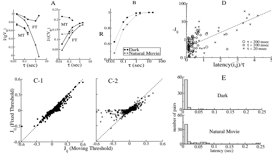
Fig. 5 Amplitudes of the interactions and currents in Dark and Natural Movie. A. Average value of the current (left) and root mean square value of the coupling (right) as a function of the membrane leaking time \tau . Points corresponding to the Fixed Threshold (FT) procedure are joined by full lines, while dashed lines indicate the results from the Moving Threshold (MT) algorithm. Note that the currents are larger in Dark than in Natural Movie. B. Correlation coefficient R (26) between the couplings at leaking time \tau and with no leakage. C. Comparison between the interactions J_{ij} found with the Moving (x-axis) and the Fixed (y-axis) Threshold procedures, for Dark (C-1) and Natural Movie (C-2). The dashed line is the x = y line, and \tau = 20 msec. D. Strongly negative couplings J_{ij} vs. latency over the membrane leaking time \tau for three values of \tau . Couplings were obtained using the Moving Threshold procedure, and correspond to the Natural Movie data set. Only interactions J_{ij} < -1 are considered; there are, respectively, 16, 28, and 60 such couplings for \tau = 200, 100, and 20 msec. The value of the slope of the best linear fit \log(-J_{ij}) = \alpha \text{ latency}(i, j)/\tau + \beta , shown by the dashed line, is \alpha = 0.95 . E. Distributions of the latencies (28) between neurons in Dark (top) and Natural Movie (bottom). Only latencies larger than 5 msec are taken into account in the histograms.
