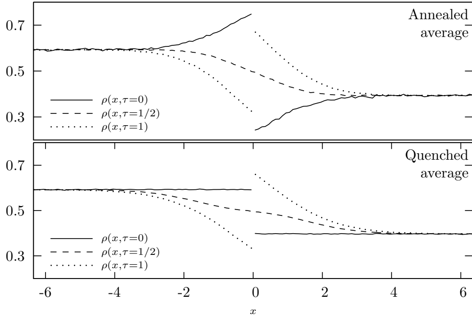
FIG. 2: Average rescaled density \rho(x, \tau) (see (14)) for the SSEP, in the annealed and quenched cases, when \lambda = 1.5 , \rho_a = 0.6 and \rho_b = 0.4 . While the initial profile is a step function in the quenched case, it deviates from it in the annealed case.
