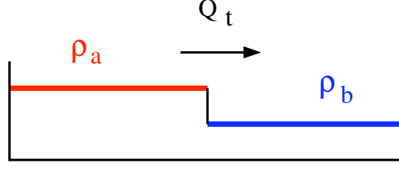
FIG. 1: The step initial condition with a density \rho_a at the left of the origin and \rho_b at the right of the origin
