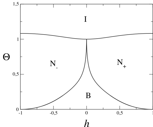
FIG. 2. Sketch of the phase diagram in the variables h (cf. (17)) and \Theta = \frac{12kT}{J\gamma r^2(h^2+3)} , where \gamma is the coordination number. The phases are isotropic (I) uniaxial nematic ( N_{\pm} ), and biaxial nematic (B).
