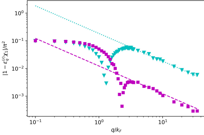
FIG. 2. Log-log representation of the mean-field (purple squares) and the RPA (turquoise triangles) numerical absolute values of the subdominant terms in \chi_1(q, \varepsilon_q^i) rescaled by the dominant O(q^{-2}) term for a mass ratio \eta = 1 . The lines represent the 1/q^3 asymptotic behaviors for mean-field (purple dashed) and RPA (dotted turquoise) associated with their respective values of \kappa [Eqs. (31) and (7)]. We see that the numerics agree with the predicted asymptotic behaviors. We see that, contrary to the MF result, RPA satisfies the asymptotic behavior required by renormalization of the polaron energy.
