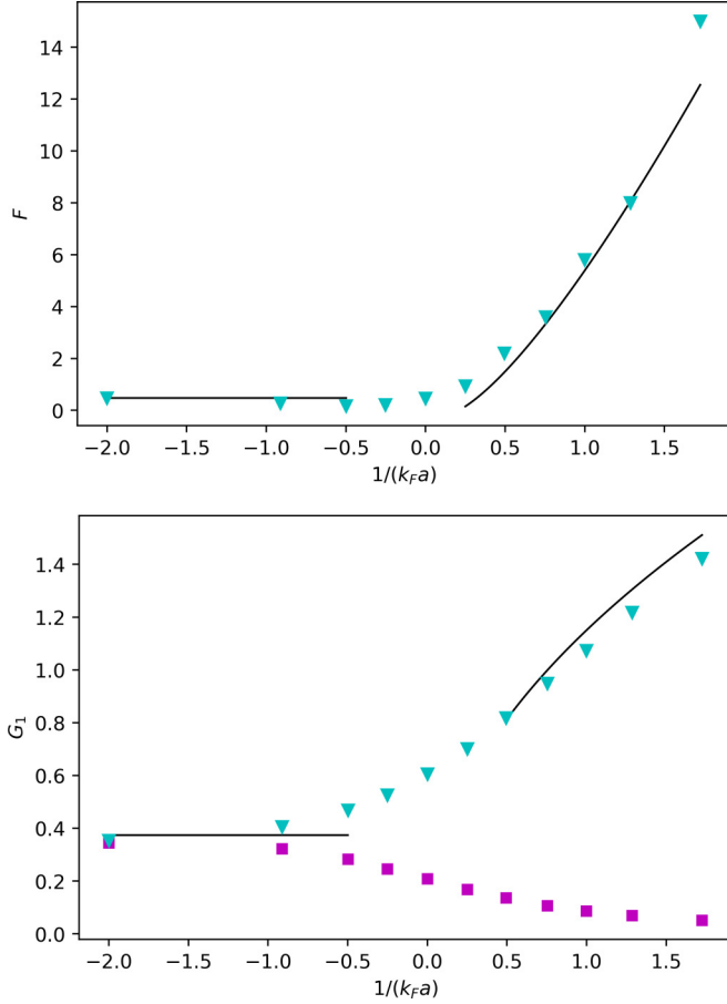
FIG. 1. Values of F (polaron energy) and G_1 (polaron mass) when the fermion-fermion interaction strength is varied. (Turquoise triangles) Numerical values using RPA for F(1/k_F a) (upper panel) and G_1 (lower panel) with \eta = 1 . The solid lines correspond to the BCS and BEC asymptotic limits, and in the lower panel the purple squares correspond to the mean-field prediction accounting only for pair-breaking excitations.
