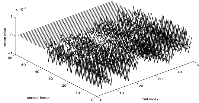
Figure 3: Changes in the different inputs when no motor commands are given and the environment changes. The first 40 sensors depend on the environment (exteroceptive) and the 20 last ones do not (proprioceptive).
