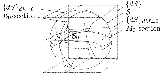
Figure 2: The sensory manifold in the neighbourhood of S_0 , the E_0 and M_0 -sections (see text). These two manifolds are transverse, and their intersection is the manifold of the sensory inputs accessible either through motion of the exteroceptive body or motion of the environment.
