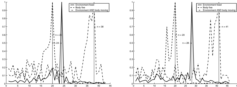
Figure 6: Dimension estimation when the diaphragm aperture is determined by reflex (left graph) and controlled by the organism (right graph). x axis is the index of the eigenvalues sorted in decreasing order of magnitude.
