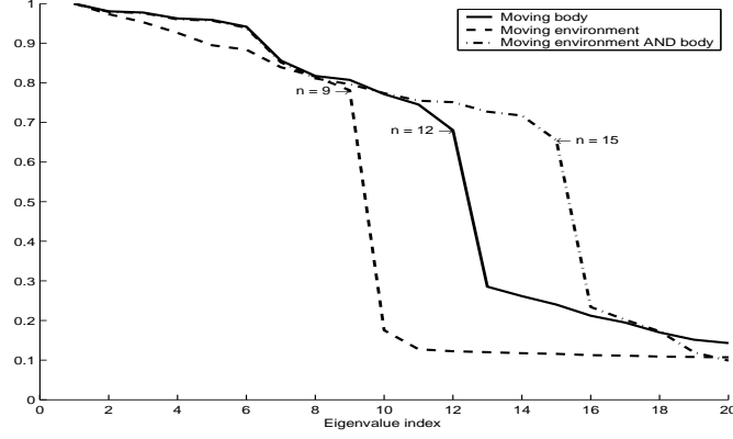
Figure 4: Eigenvalues of the covariance matrices in the three cases described in the text, ordered in decreasing rank order (normalized log scale). The dimensions of the tangent spaces are taken to be equal to the number of significantly non-zero eigenvalues (see Figure 5).
