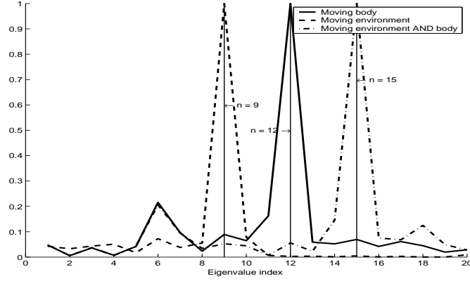
Figure 5: Ratio of successive eigenvalues i and i+1 (normalized logarithmic scale). The number of dimensions is taken as the number of eigenvalues up to and including the maximum of this ratio (see Appendix). We could also have used an approach similar to Minka, 2000.
