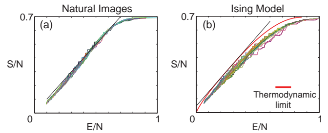
FIG. 3 (color). Indication of critical behavior in the plot of entropy vs energy. (a) The results for rectangular image patches of size 8 to 50 pixels (different colors). (b) Results for Monte Carlo simulations of the 2D Ising model.
