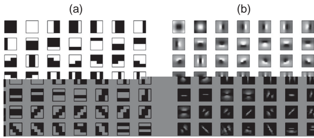
FIG. 4. Locally stable states. (a) The 49 most probable patches such that all single pixel inversions decrease their probability in the ensemble. Even in small ( 4 \times 4 ) patches these locally stable states are interpretable as lines and edges at all positions and orientations. (b) The average surrounding 10 \times 10 light-intensity images leading to these metastable states. These images resemble the average images that trigger responses of neurons in primary visual cortex.
